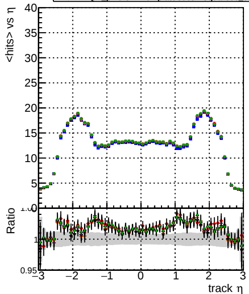
mean hit BOW original step2 tbar-phase1-newgeom BOW pixel CDF template CutChiSquare10 step2 tbar-phase1-newgeom BOW pixel CDF template CutChiSquare15 step2 tbar-phase1-newgeom BOW pixel CDF template CutChiSquare30 step2 tbar-phase1-newgeom
