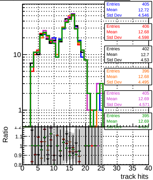
mean hit BOW original step2 template cutChiSquare10 step2 tbar-phase1-newgeom BOW pixel CDD template cutChiSquare15 step2 tbar-phase1-newgeom BOW pixel CDD template cutChiSquare30 step2 tbar-phase1-newgeom
