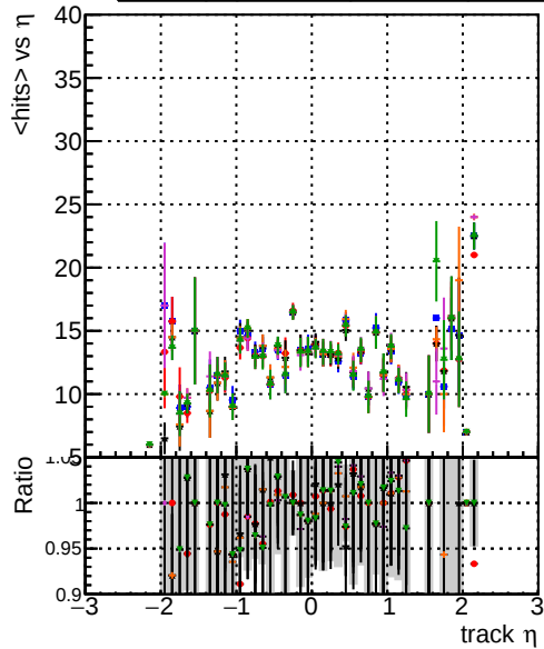
mean hit BOW original step2 template cutChiSquare10 step2 tbar-phase1-newgeom BOW pixel CDD template cutChiSquare15 step2 tbar-phase1-newgeom BOW pixel CDD template cutChiSquare30 step2 tbar-phase1-newgeom
