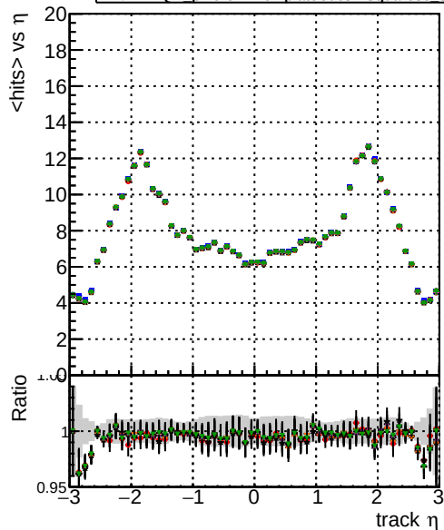
Legend: BDM original, BDM pixel, BDM pixel CDD, BDM pixel CDD template, BDM pixel CDD template cut, BDM pixel CDD template cut chi square, BDM pixel CDD template cut chi square step 2, BDM pixel CDD template cut chi square step 2 tbar phase 1 newgeom, BDM pixel CDD template cut chi square step 2 tbar phase 1 newgeom
