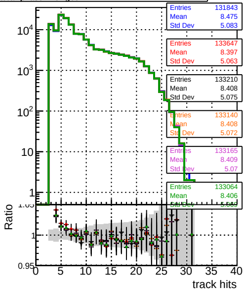
Legend: BDM original, BDM pixel, BDM pixel CDD, BDM pixel CDD template, BDM pixel CDD template cut, BDM pixel CDD template cut chi square, BDM pixel CDD template cut chi square step 2, BDM pixel CDD template cut chi square step 2 tbar phase 1 newgeom, BDM pixel CDD template cut chi square step 2 tbar phase 1 newgeom
