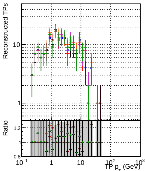
N of sim DOM original_step2_tbar-phase1-newgeom pixetemplate_square10_step2_tbar-phase1-newgeom pixetemplate_square15_step2_tbar-phase1-newgeom pixetemplate_square20_step2_tbar-phase1-newgeom pixetemplate_square30_step2_tbar-phase1-newgeom
