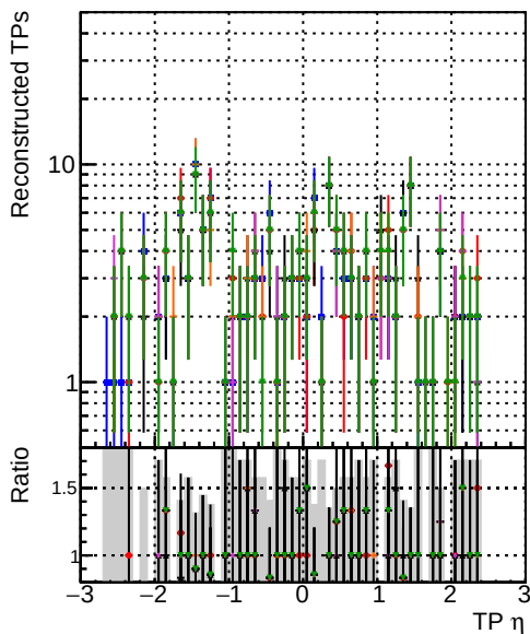
N of sim DOM original_step2_tbar-phase1-newgeom pixetemplate_square10_step2_tbar-phase1-newgeom pixetemplate_square15_step2_tbar-phase1-newgeom pixetemplate_square20_step2_tbar-phase1-newgeom pixetemplate_square30_step2_tbar-phase1-newgeom
