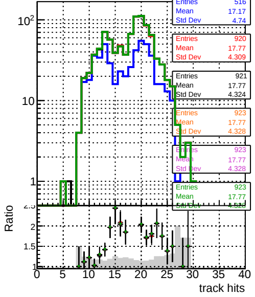
mean hit
