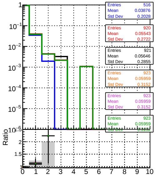
mean hit
