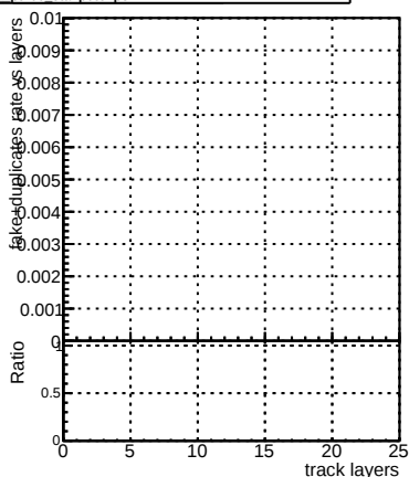
pt200_eta2p0to2p5 pt200_eta2p0to2p5 pt200_eta2p0to2p5
