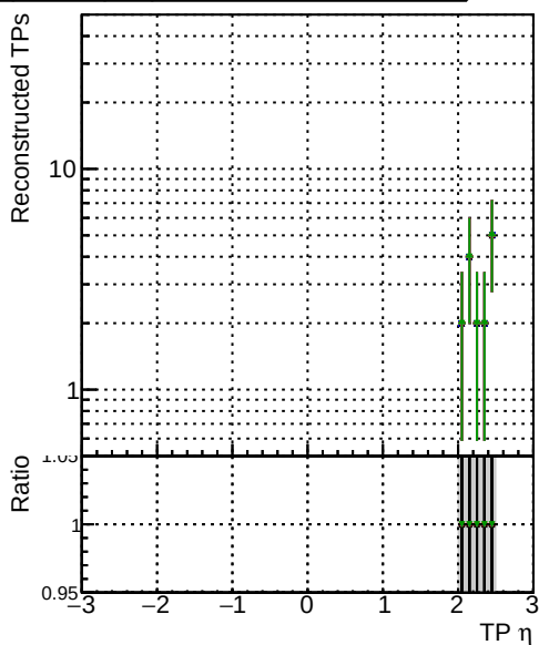
DOM original step2 eta200 eta2p0t02p5 N of sim DOM pixel CPE template step2 p1200 eta2p0t02p5 DOM pixel CPE template CutChiSquare15 step2 p1200 eta2p0t02p5 DOM pixel CPE template CutChiSquare20 step2 p1200 eta2p0t02p5 DOM pixel CPE template CutChiSquare20 step2 p1200 eta2p0t02p5 DOM pixel CPE template CutChiSquare30 step2 p1200 eta2p0t02p5
