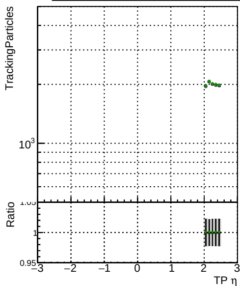
DOM original step2 eta200 eta2p0t02p5 N of sim DOM pixel CPE template step2 p1200 eta2p0t02p5 DOM pixel CPE template CutChiSquare15 step2 p1200 eta2p0t02p5 DOM pixel CPE template CutChiSquare20 step2 p1200 eta2p0t02p5 DOM pixel CPE template CutChiSquare20 step2 p1200 eta2p0t02p5 DOM pixel CPE template CutChiSquare30 step2 p1200 eta2p0t02p5
