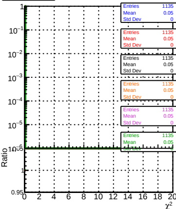
normalized \chi^2
