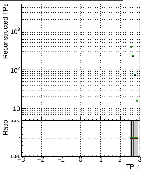
pt1to20-eta2p5f04p00 pt1to20-eta2p5f04p00
