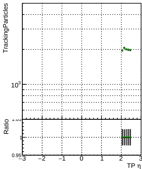
N of sim Model Pixel CPTE Template Cut ChiSquare Step bf1to20 eta20to25 bf1to20 eta20to25 1 DOM pixel CPTE Template Cut ChiSquare15 Step2 bf1to20 eta20to25 bf1to20 eta20to25 2 DOM pixel CPTE Template Cut ChiSquare20 Step3 bf1to20 eta20to25 bf1to20 eta20to25 3 DOM pixel CPTE Template Cut ChiSquare20 Step3 bf1to20 eta20to25 bf1to20 eta20to25 4 DOM pixel CPTE Template Cut ChiSquare30 Step2 bf1to20 eta20to25 bf1to20 eta20to25
