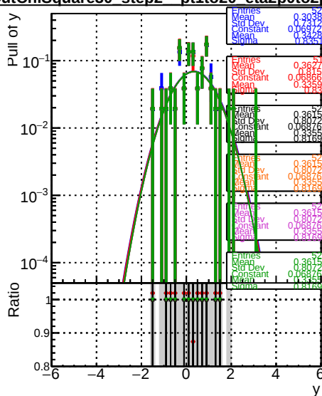
RecoAllAssoc2GenMatched_PullY
