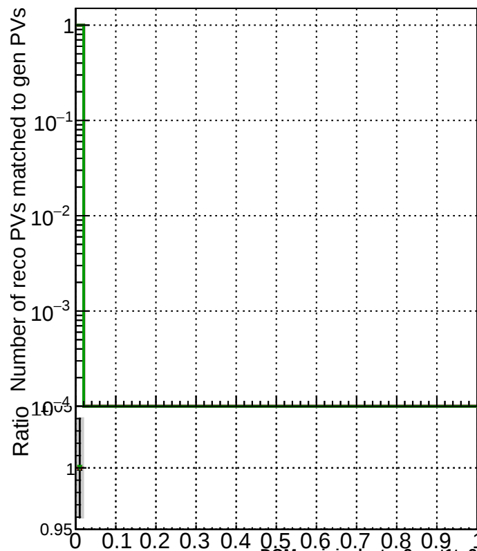
RecoPVAssoc2GenPVMatched_Purity
