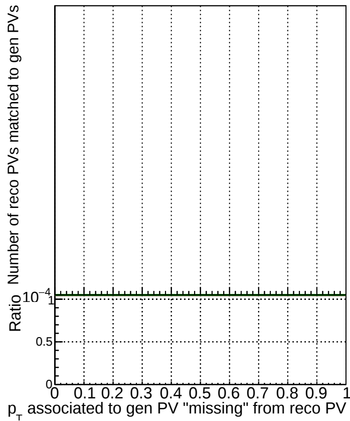
RecoPVAssoc2GenPVMatched_missing
