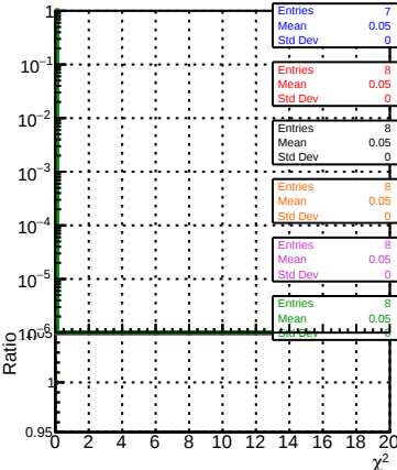
normalized \chi^2
