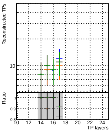
pt1to20_eta1p6to2p0 pt1to20_eta1p6to2p0 pt1to20_eta1p6to2p0
