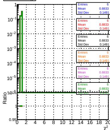
normalized \chi^2
