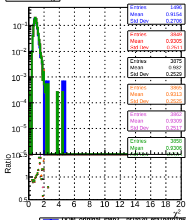
normalized \chi^2
