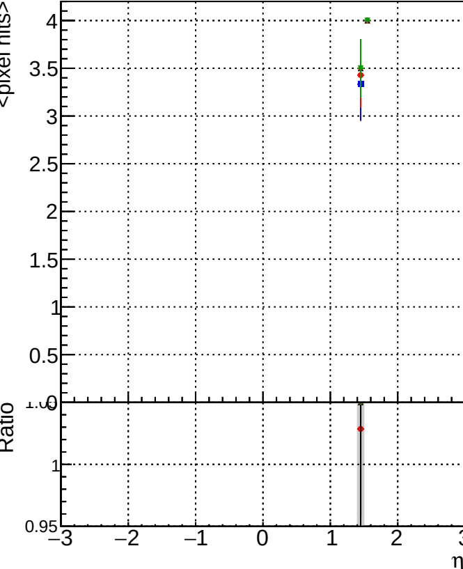
original step2 pt1to20 eta1p4to1p6 DQM pixelCPEtemplate step2 pt1to20 eta1p4to1p6 DQM pixelCPEtemplate CutChiSquare10 step2 pt1to20 DQM pixelCPEtemplate CutChiSquare15 step2 pt1to20 DQM pixelCPEtemplate CutChiSquare20 step2 pt1to20 DQM pixelCPEtemplate CutChiSquare30 step2 pt1to20
