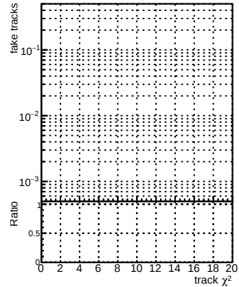
N of fake tracks vs normalized \chi^2
