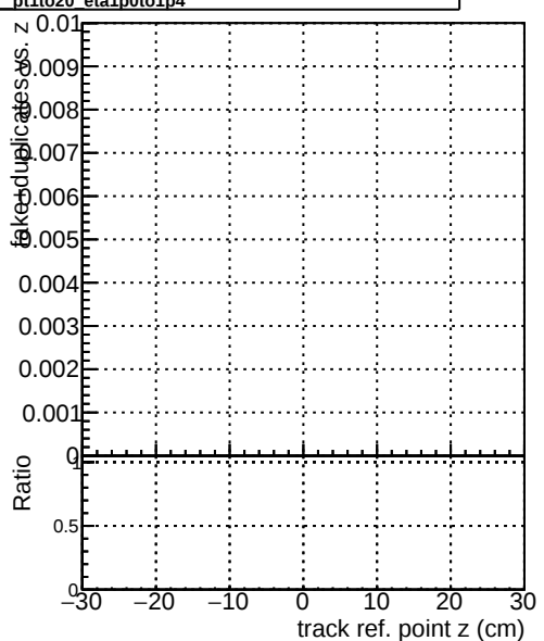
pt1to20-eta1b0to1p4 pt1to20-eta1b0to1p4 pt1to20-eta1b0to1p4
