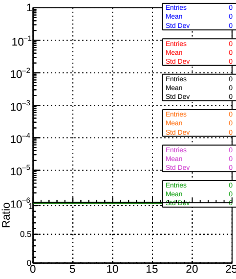
mean hit original step2 p1to1000 eta2p6to4p0 CDT template CutsChiSquare10 step2 p1to1000 eta2p6to4p0 CDT template CutsChiSquare15 step2 p1to1000 eta2p6to4p0 CDT template CutsChiSquare20 step2 p1to1000 eta2p6to4p0 CDT template CutsChiSquare30 step2 p1to1000 eta2p6to4p0
