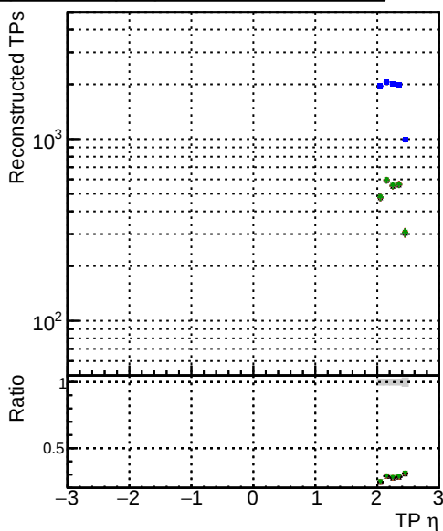
pt1to1000-eta2p0to2p5
