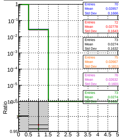
Legend for mean hits vs \eta : DDV original DDV pixel DDV pixel CDD DDV pixel CDD Template DDV pixel CDD Template Cut DDV pixel CDD Template Cut Chi Square DDV pixel CDD Template Cut Chi Square 10 steps DDV pixel CDD Template Cut Chi Square 15 steps DDV pixel CDD Template Cut Chi Square 20 steps DDV pixel CDD Template Cut Chi Square 30 steps DDV pixel CDD Template Cut Chi Square 10 steps eta2p0to2p5 DDV pixel CDD Template Cut Chi Square 15 steps eta2p0to2p5 DDV pixel CDD Template Cut Chi Square 20 steps eta2p0to2p5 DDV pixel CDD Template Cut Chi Square 30 steps eta2p0to2p5
