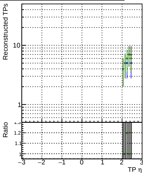
pt1to1000-eta2p0to2p5 pt1to1000-eta2p0to2p5
