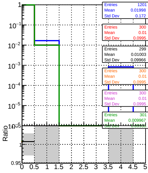
mean hits vs \eta Legend: BOW original step2 pTto1000 eta2p0to2p5 (blue), BOW pixel template CutChiSquare10 step2 pTto1000 eta2p0to2p5 (red), BOW pixel template CutChiSquare10 step2 pTto1000 eta2p0to2p5 (green), BOW pixel template CutChiSquare10 step2 pTto1000 eta2p0to2p5 (orange), BOW pixel template CutChiSquare10 step2 pTto1000 eta2p0to2p5 (purple), BOW pixel template CutChiSquare10 step2 pTto1000 eta2p0to2p5 (brown)
