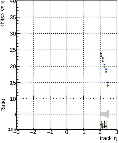
mean hits vs \eta Legend: BOW original step2 pTto1000 eta2p0to2p5 (blue), BOW pixel template CutChiSquare10 step2 pTto1000 eta2p0to2p5 (red), BOW pixel template CutChiSquare10 step2 pTto1000 eta2p0to2p5 (green), BOW pixel template CutChiSquare10 step2 pTto1000 eta2p0to2p5 (orange), BOW pixel template CutChiSquare10 step2 pTto1000 eta2p0to2p5 (purple), BOW pixel template CutChiSquare10 step2 pTto1000 eta2p0to2p5 (brown)
