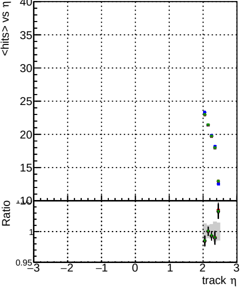
mean hits vs \eta Legend: BOW original, step2, p1to1000, eta2p0to2p5, BOW pixel, CDE template, CutChiSquare10, step2, p1to1000, eta2p0to2p5, BOW pixel, CDE template, CutChiSquare15, step2, p1to1000, eta2p0to2p5, BOW pixel, CDE template, CutChiSquare20, step2, p1to1000, eta2p0to2p5, BOW pixel, CDE template, CutChiSquare30, step2, p1to1000, eta2p0to2p5
