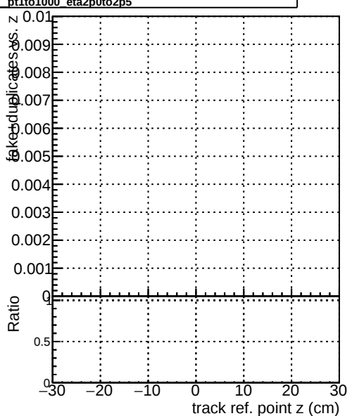
pt1to1000-eta2p0to2p5
