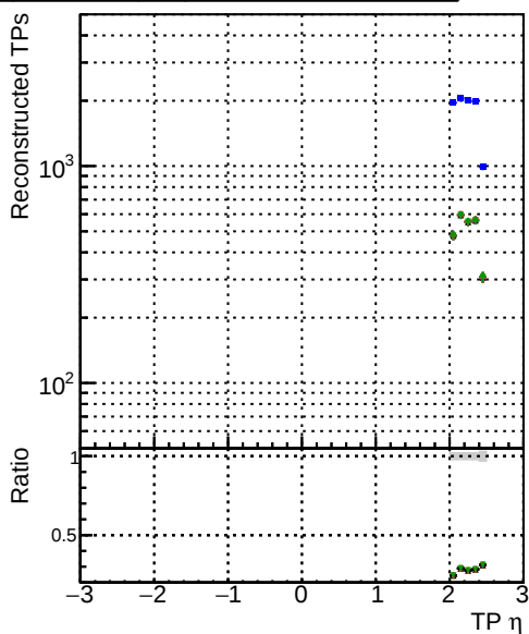
pt1to1000-eta2p0to2p5
