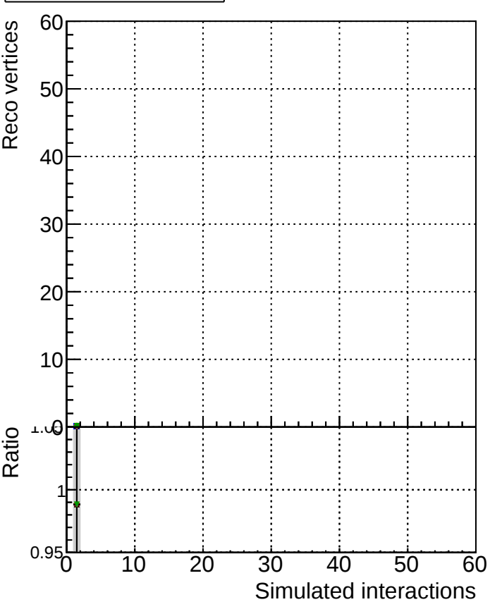
RecoVtx_vs_GenVtx
