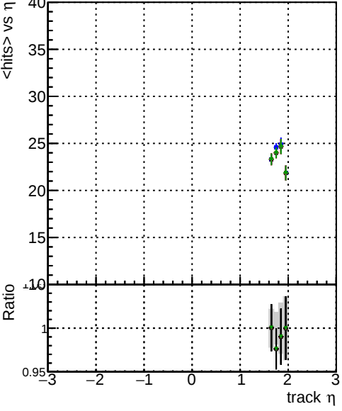
mean hits vs \eta Legend: BQM original step2 pTto1000 eta1p6to2p0 BQM pixel CDF template CutChiSquare10 step2 pTto1000 eta1p6to2p0 BQM pixel CDF template CutChiSquare15 step2 pTto1000 eta1p6to2p0 BQM pixel CDF template CutChiSquare20 step2 pTto1000 eta1p6to2p0 BQM pixel CDF template CutChiSquare30 step2 pTto1000 eta1p6to2p0
