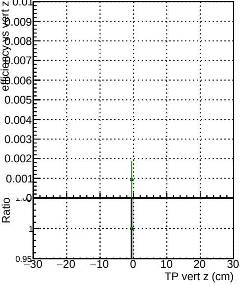
Efficiency vs vert z Legend: BDV original Step 2 eta1p6to2p0 BDV pixelCUT TemplateCutChiSquare10 Step2 eta1p6to2p0 BDV pixelCUT TemplateCutChiSquare15 Step2 eta1p6to2p0 BDV pixelCUT TemplateCutChiSquare20 Step2 eta1p6to2p0 BDV pixelCUT TemplateCutChiSquare30 Step2 eta1p6to2p0
