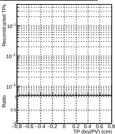
pt1to1000_eta1p6to2p0 pt1to1000_eta1p6to2p0 pt1to1000_eta1p6to2p0
