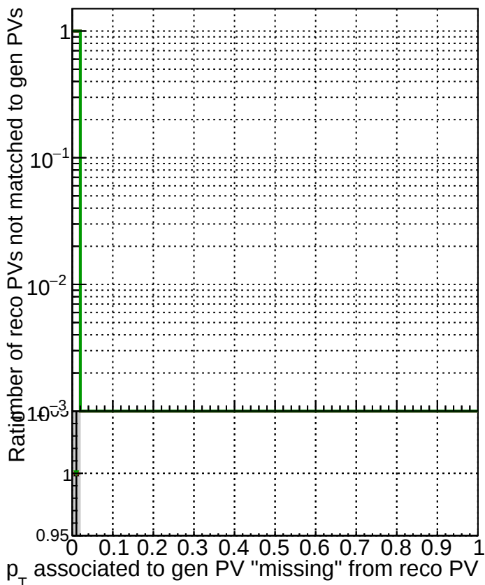
es0_stepz__pl1l01000_elalp4l0lp0 RECOPVASSUCZGENPVINOTmatched_missing
