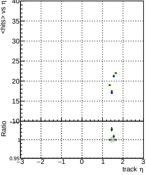
mean hits vs \eta Legend: BGM original, step2, eta1to1000, eta1p4to1p6, BGM pixel, CDP, TemplateCut, ChiSquare10, step2, eta1to1000, eta1p4to1p6, BGM pixel, CDP, TemplateCut, ChiSquare30, step2, eta1to1000, eta1p4to1p6
