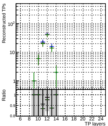
pt1to1000_eta1p0to1p4 pt1to1000_eta1p0to1p4 pt1to1000_eta1p0to1p4
