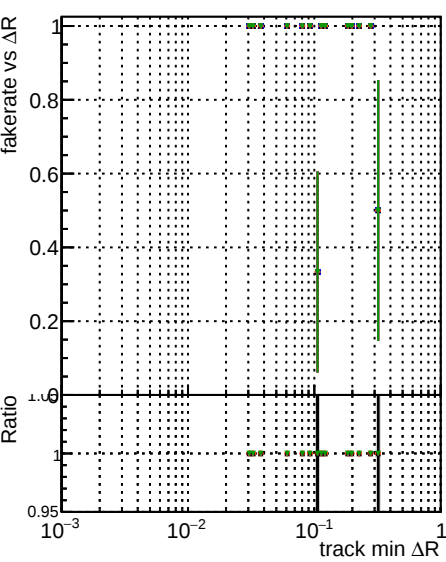
Fake rate vs \Delta R(\text{track, jet}) Legend: DOM (blue), original (red), step2 (green), pt1to1000 (purple), eta1to1p4 (brown), pt1to1000_eta1to1p4 (pink), and a baseline (black).
