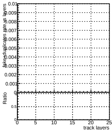
pt1to1000_eta1p0to1p4 pt1to1000_eta1p0to1p4
