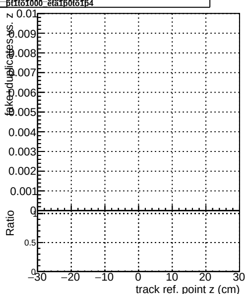
pt1to1000-eta1p0to1p4 pt1to1000-eta1p0to1p4 pt1to1000-eta1b0to1b4
