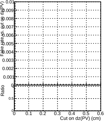
Fake rate
