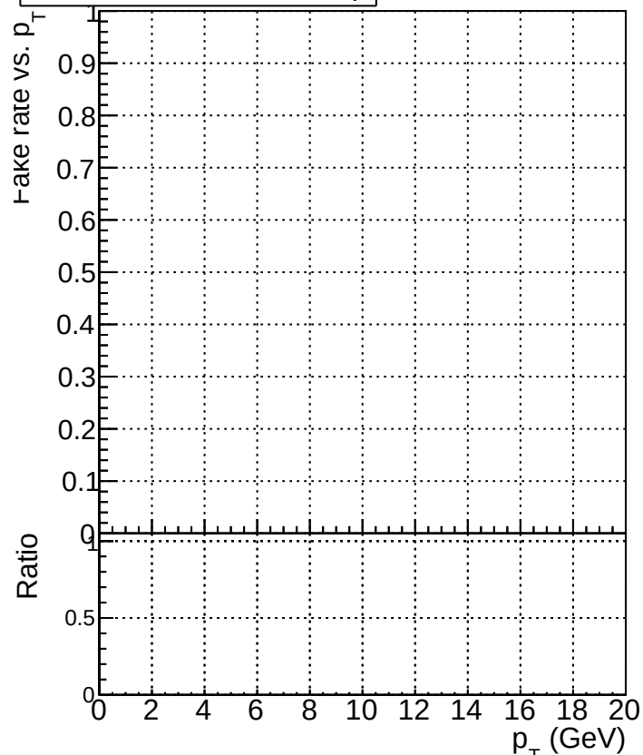
K S 0 tracking fake rate vs p T
