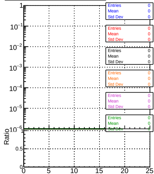
Legend for mean hits vs \eta : Blue: BGM original Red: BGM original + step2 Black: BGM original + step2 + 1000 Orange: BGM original + step2 + 1000 + eta2p0to2p5 Green: BGM original + step2 + 1000 + eta2p0to2p5 + BGM template
