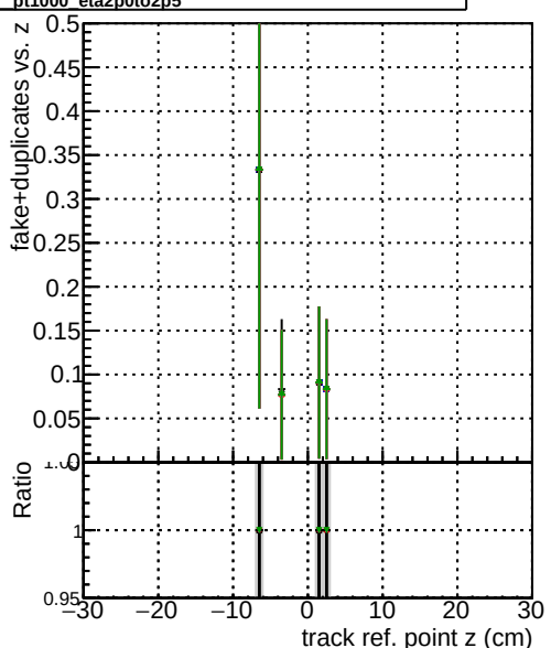
pt10000-eta20010205 pt10000-eta20010205 pt10000-eta20010205
