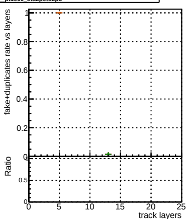
pt1000_eta2p0to2p5 pt1000_eta2p0to2p5 pt1000_eta2p0to2p5
