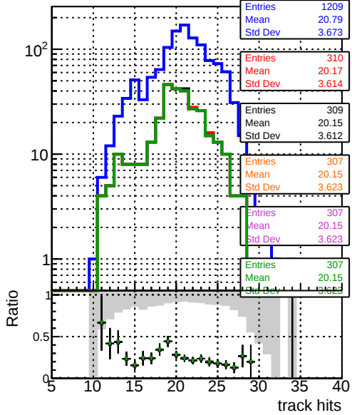
mean hit BDW original step2 pt1000 eta2p0to2p5 BDW pixel step2 pt1000 eta2p0to2p5 BDW pixel CDF step2 pt1000 eta2p0to2p5 BDW pixel CDF Template step2 pt1000 eta2p0to2p5 BDW pixel CDF Template Cut Chi Square step2 pt1000 eta2p0to2p5 BDW pixel CDF Template Cut Chi Square step2 pt1000 eta2p0to2p5 BDW pixel CDF Template Cut Chi Square step2 pt1000 eta2p0to2p5
