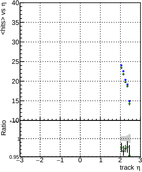
mean hit BDW original step2 pt1000 eta2p0to2p5 BDW pixel step2 pt1000 eta2p0to2p5 BDW pixel CDF step2 pt1000 eta2p0to2p5 BDW pixel CDF Template step2 pt1000 eta2p0to2p5 BDW pixel CDF Template Cut Chi Square step2 pt1000 eta2p0to2p5 BDW pixel CDF Template Cut Chi Square step2 pt1000 eta2p0to2p5 BDW pixel CDF Template Cut Chi Square step2 pt1000 eta2p0to2p5
