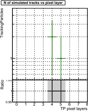
N of simulated tracks vs pixel layer
