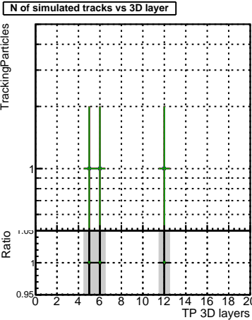
N of simulated tracks vs 3D layer
