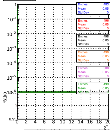
normalized \chi^2
