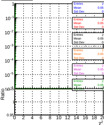
normalized \chi^2
