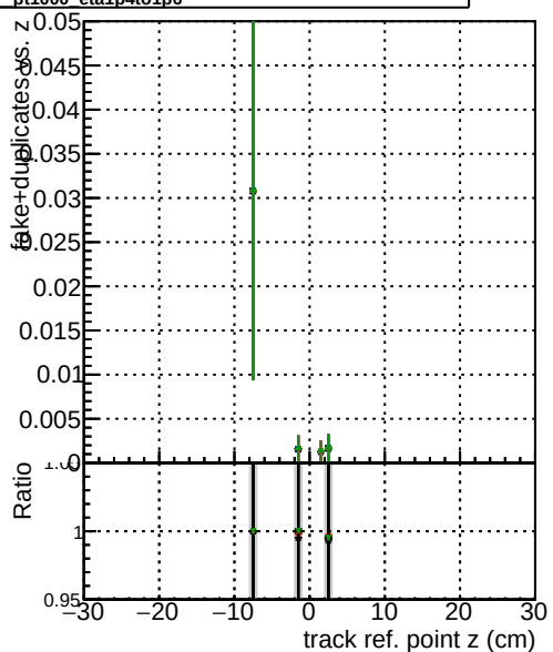
pt1000-eta1p4t01p6 pt1000-eta1p4t01p6 pt1000-eta1p4t01p6
