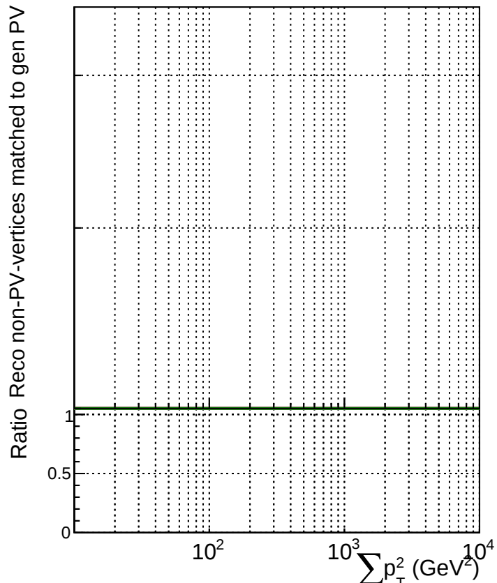
RecoAssoc2GenPVMatchedNotHighest_Pt2
