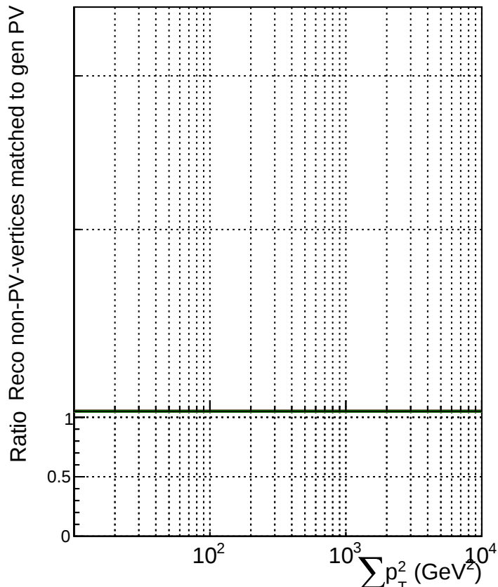
RecoAssoc2GenPVMatchedNotHighest_Pt2
