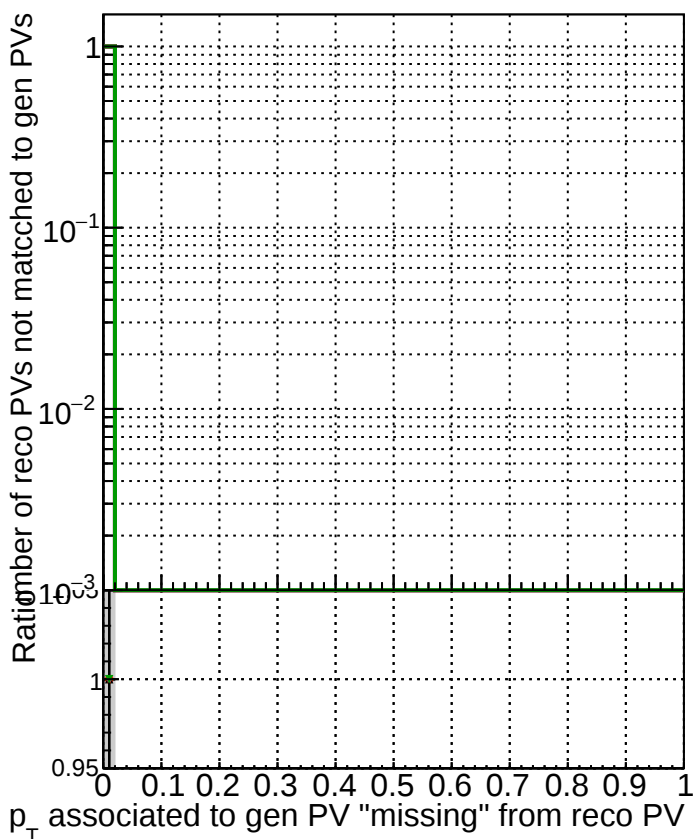
es0_stepz_pli000_elaipl0l0lp4 RECOPVASSOCZGENPVNOTmatched_missing
